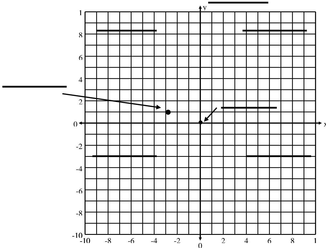
Rectangular Coordinate System
