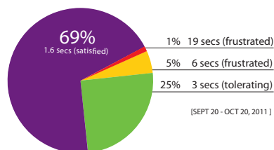
Average Latency and User Satisfaction
